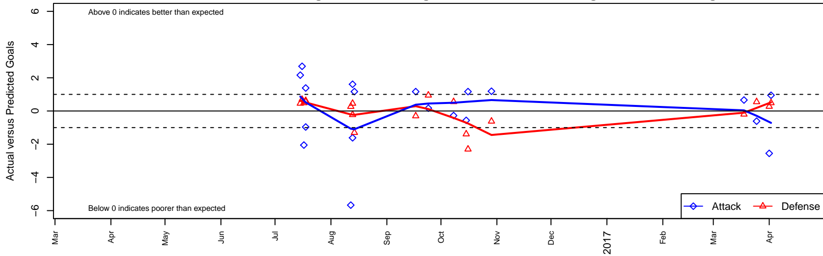
Spokane Sounders A North G05 Dots are actual minus expected GF (blue circles) and GA (red triangles). Blue line is smoothed change in attack strength. Red is smoothed change in defense strength.
